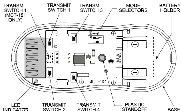
Figure 3. Component Layout
